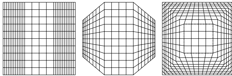
2 Distortion patterns found in Bifocal Display (left), Perspective Wall (center), and Document Lens (right).
